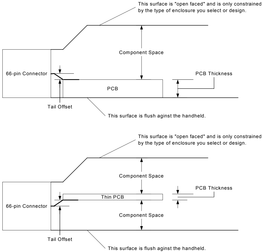
Figure 7-2. Connector Considerations
